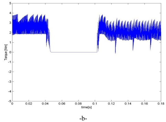
Fig.5 Dynamic responses of SRM with DTC a- Current and b- Torque
